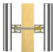
Back-to-back fix An internal and external pull bar hiding the fixing within the door application
